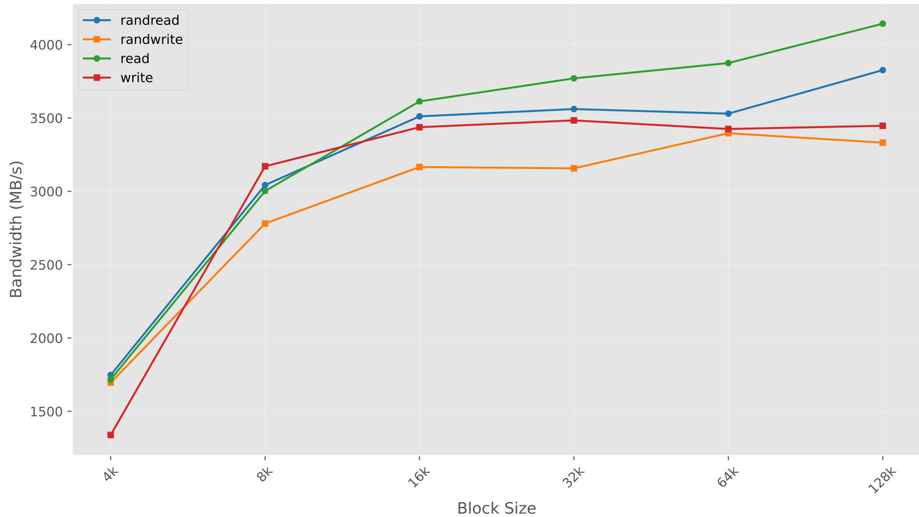
Bandwidth vs Block Size
